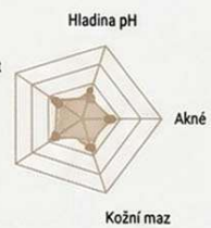
Pigmentace dermis
